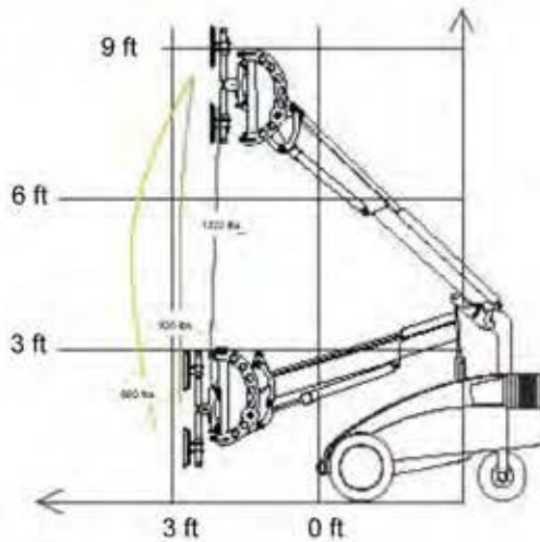
REACH DIAGRAM
