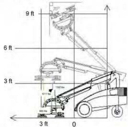
PICKUP AND PLACE DIAGRAM
