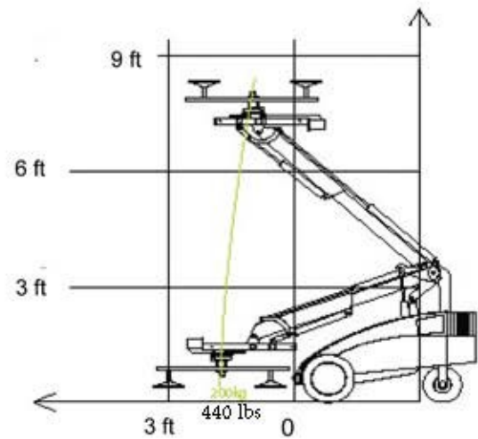
PICKUP AND PLACE DIAGRAM
